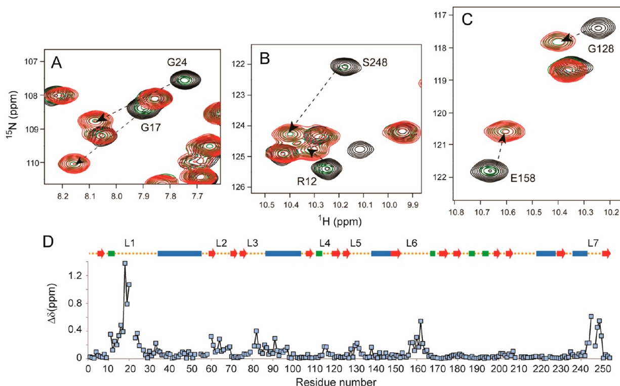
Figure 3. NMR titration of TM-PaDDAH with L-citrulline. (A–C) Selected regions of the ^{15}\text{N} , ^1\text{H} -HSQC spectrum of 0.3 mM TM-PaDDAH recorded in the presence of different concentrations of L-citrulline. Dashed arrows indicate the chemical shift perturbation from the spectrum of the apo protein (black) to the effectively saturated complex (red). The concentration of L-citrulline in each spectrum was 0 mM (black), 0.18 mM (dark green), and 0.46 mM (red), respectively. (D) Combined chemical shift ^{15}\text{N} , ^1\text{H} perturbation ( \Delta\delta ) plotted as a function of residue number. The secondary structure of PaDDAH is depicted at the top of the graph.
