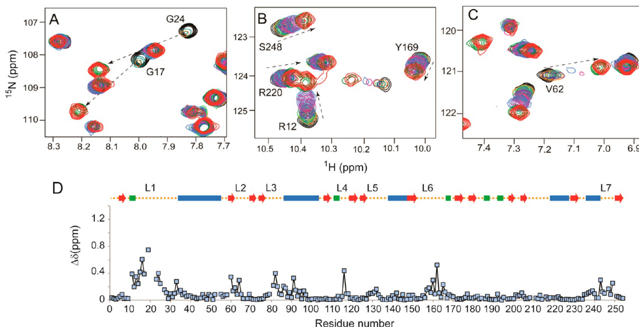
Figure 2. NMR titration of DM-PaDDAH with L-citrulline. (A–C) Selected regions of the ^{15}\text{N} , ^1\text{H} -HSQC spectrum of 0.3 mM DM-PaDDAH recorded in the presence of different concentrations of L-citrulline. Dashed arrows indicate the chemical shift perturbation from the spectrum of the apo protein (black) to the effectively saturated complex (red). The concentration of L-citrulline in each spectrum was 0 mM (black), 0.6 mM (teal), 1.8 mM (orange), 3.0 mM (light green), 5.4 mM (purple), 8.7 mM (magenta), 13.8 mM (blue), 15.9 mM (dark green), and 20.7 mM (red), respectively. (D) Combined chemical shift ^{15}\text{N} , ^1\text{H} perturbation ( \Delta\delta ) plotted as a function of residue number. The secondary structure of PaDDAH is depicted at the top of the graph. The vertical scale is matched to that of Figure 3D. Values of \Delta\delta for residues Leu18 and Ser20 were not measurable as the bound-state cross peaks are broadened beyond detection even at the highest loading of L-citrulline.
