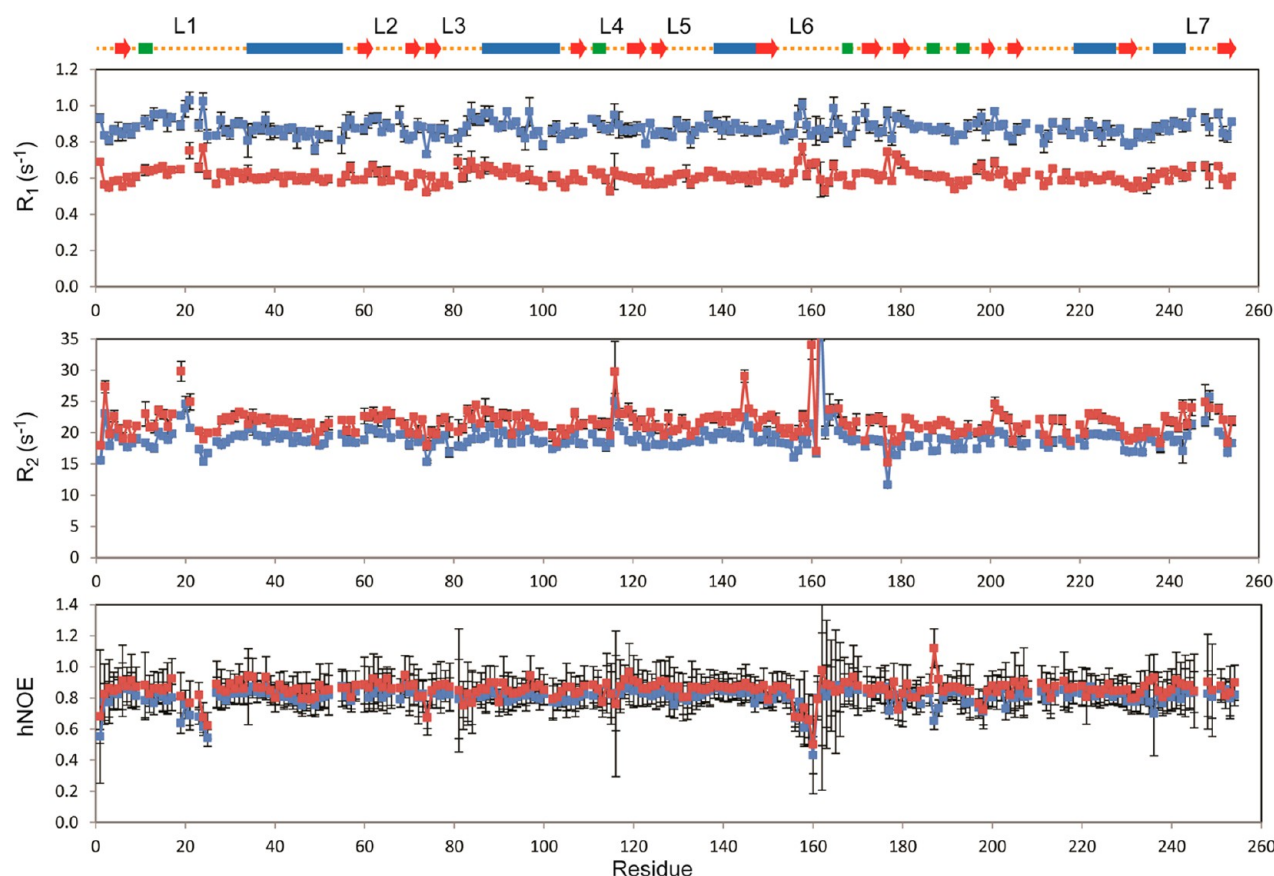
Figure 6. ^{15}\text{N} nuclear relaxation measurements for L-citrulline-saturated DM-PaDDAH. Per-residue ^{15}\text{N} R_1 , ^{15}\text{N} R_2 , and \{^1\text{H}\}^{15}\text{N} heteronuclear NOE (hNOE) values obtained at ^1\text{H} 600 MHz (blue) and 800 MHz (red) and 25 °C. The secondary structure of PaDDAH is depicted at the top of the figure.
