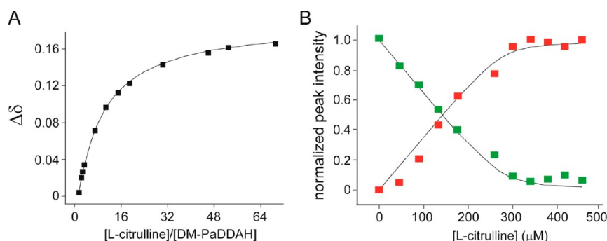
Figure 4. Ligand-dependent effects on the NMR spectrum of DM- and TM-PaDDAH proteins. Nonlinear best fits of the L-citrulline-dependent change in (A) combined ^{15}\text{N} , ^1\text{H} chemical shifts and (B) apo (green squares) and bound (red squares) cross peak intensities for 0.3 mM DM-PaDDAH and TM-PaDDAH, respectively. In each case, data points are aggregated over a small number of well-resolved cross peaks. The fitted values of the DM-PaDDAH/L-citrulline and TM-PaDDAH/L-citrulline dissociation constants are K_D^{(\text{DM/L-cit})} = 3.6 \pm 0.1 mM and K_D^{(\text{TM/L-cit})} = 3.5 \pm 1.5 \mu\text{M} , respectively.
