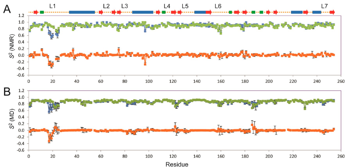
Figure 7. NMR and MD-derived order parameters for apo and L-citrulline-bound DM-PaDDAH. (A) Plots of the generalized order parameters S^2 for ^{15}\text{N} – ^1\text{H} bond vector orientations obtained by model-free analysis of the multiple field ^{15}\text{N} R_1 , R_2 , and \{^1\text{H}\}^{15}\text{N} heteronuclear NOE data for apo (blue) and L-citrulline-saturated (green) DM-PaDDAH. (B) Plots of ^{15}\text{N} – ^1\text{H} S^2 values obtained from multiple slices of molecular dynamics trajectories computed for apo (blue) and L-citrulline-saturated (green) DM-PaDDAH based upon the crystal structure coordinates PDB code 1H70. In both (A) and (B), the difference in S^2 values between the two states is plotted in orange. The secondary structure of PaDDAH is depicted at the top of the figure.
