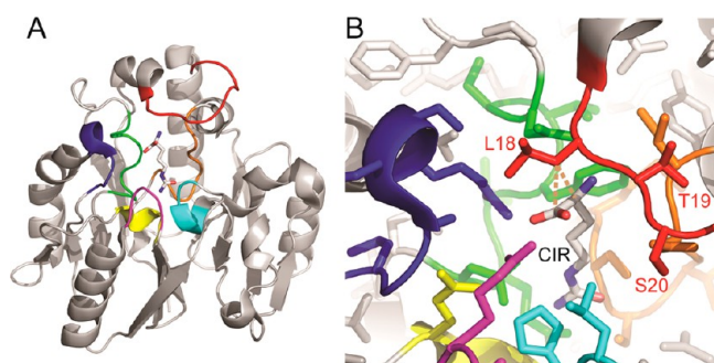
Figure 1. Three-dimensional structure of PaDDAH bound to L-citrulline showing the main features relevant to this work. (A) Ribbon representation of the crystal structure (PDB code 1H70) of the Cys249Ser mutant PaDDAH bound to L-citrulline. The ligand is shown in stick form with standard atom-type coloring. Loops that surround the active site chamber are depicted in color: red, loop 1 (L1); green, L2; blue, L3; yellow, L4; magenta, L5; cyan, L6; and orange, L7. (B) Close-up of the coordination of L-citrulline (CIR) by PaDDAH side chains. Protein side chain atoms (only) are displayed in stick representation and the color scheme is as in (A). The side chains of Leu18, Thr19, and Ser20 in L1 are labeled. Dashed lines (brown) indicate the van der Waals contact between the C \beta of Leu18 and the C \alpha and carboxylate carbon atoms of the ligand.
